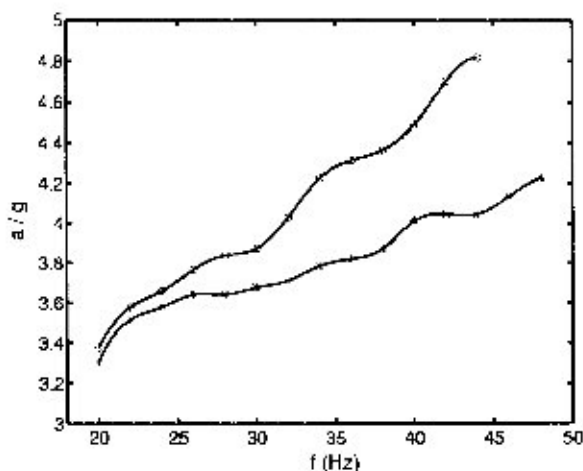
Fig. 6. The threshold (in units of g) for hexagonal lattice as a function of frequency f for 20 g (symbol ○) and 10 gms (symbol *) of pure alumina. The line is only a guide to eyes.
