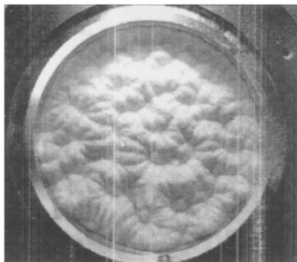
Fig. 3. A typical case of interacting heaps at a = 5.5g ( g is the acceleration due to gravity), f = 42 Hz for 40 g of alumina showing a spatio-temporal pattern.
