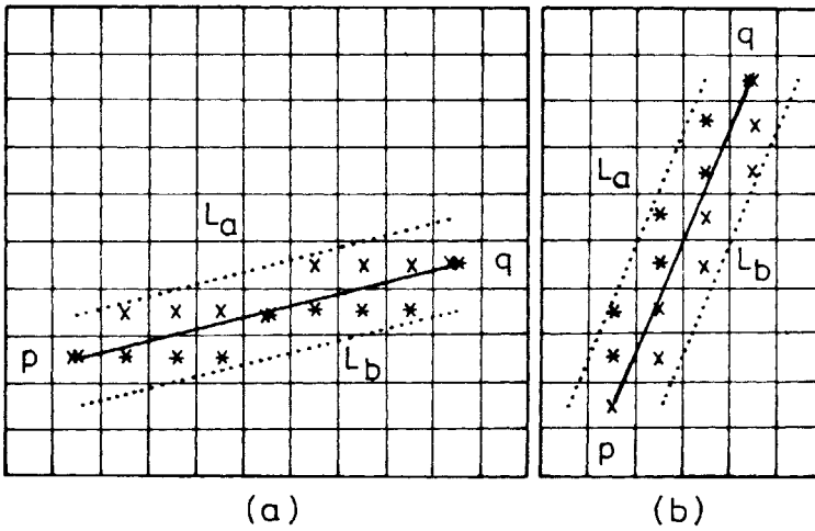
FIG. 2. Digital straight line segment connecting p and q . L_a consists of pixels marked with 'x' and L_b consists of pixels marked with '*'.
