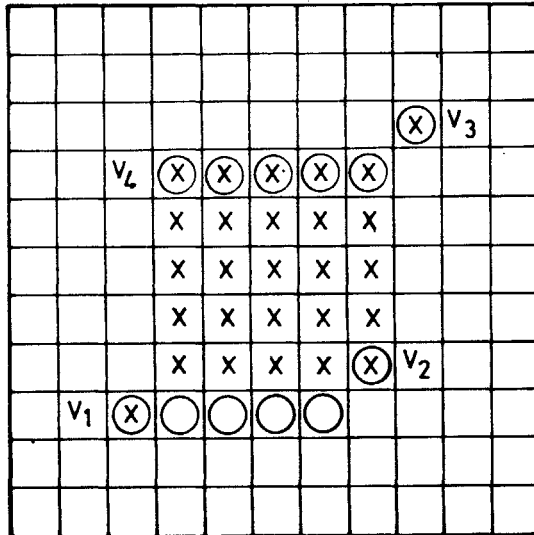
FIG. 12. A simply connected convex object.
