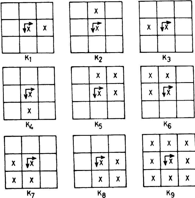
FIG. 5. Structuring elements for Yokoi connectivity number for 4-connectivity.
