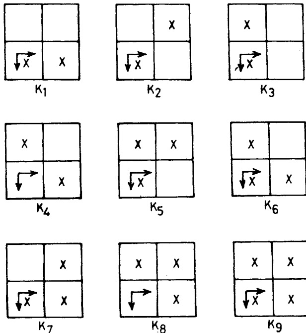
FIG. 9. Structuring elements for computing genus for 8-connectivity.
