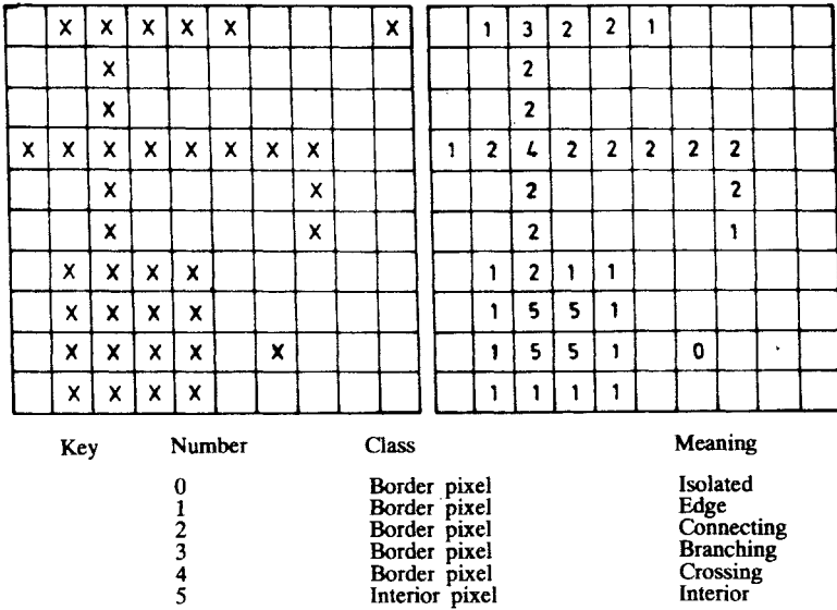
Fig. 4. Illustration of a connectivity number labeling of a binary image 5 .
