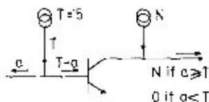
Fig. 3. Threshold detector.
