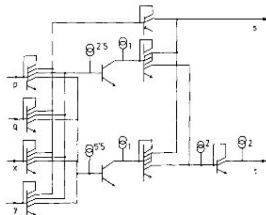
Fig. 4. Mapped balanced ternary four-sum and adder.
