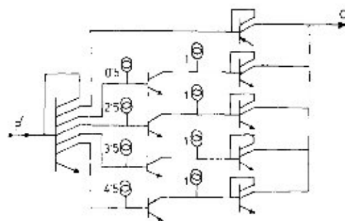
Fig. 6. Circuit for generation of carry C from P^i .
