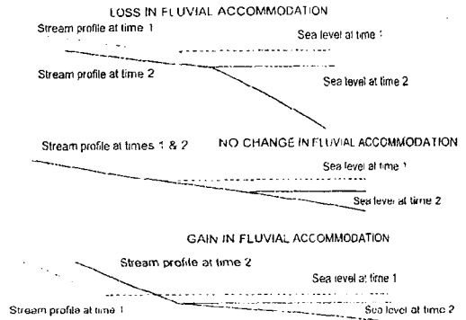
Fig. 12 Changes in fluvial accommodation in response to relative sea level fall under three different conditions of relative gradients between stream and shelf profiles.
