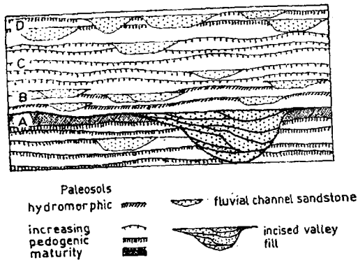
Fig. 14 Paleosol characteristics under different conditions of accommodation space creation in a sedimentary succession. The level A denotes little or no accommodation space generation signifying an unconformity and period of landscape stability. The rate of accommodation creation is highest in the level B leading to development of hydromorphic paleosols, which gradually decreases upwards resulting in increasing pedogenic maturity from level C to D. Adopted from Kraus (1999).
