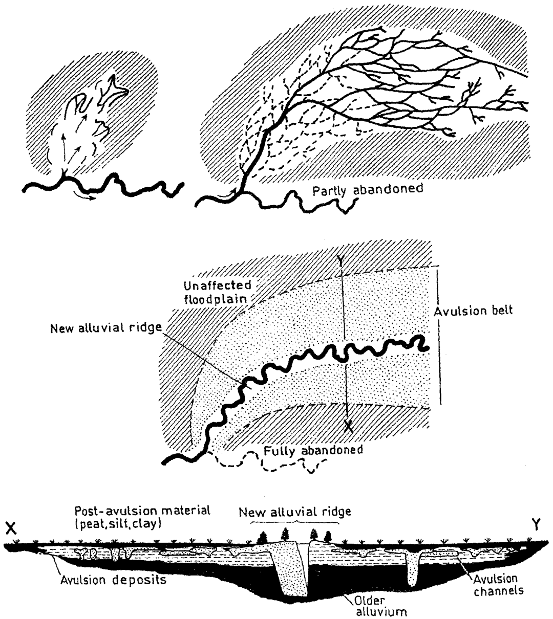
Fig. 10 Evolutionary pattern of a channel avulsion through the formation and enlargement of a crevasse lobe. Crevassing initially form an extensive belt of avulsion deposit with a network of crevasse channels within the floodplain. Smaller channels gradually evolve into a major channel and associated alluvial ridge till the next avulsion is initiated. (Modified after Smith et al., 1989).
