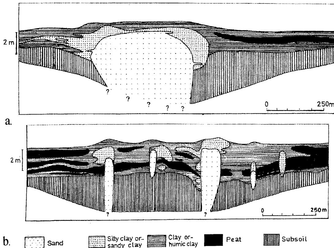
Fig. 9 Facies architecture in Holocene meander (a) and anastomosed (b) river deposits of the Rhine-Meuse Delta. Meander rivers are characterised by wider channel deposits (sand) and extensive wedge-shaped levee deposits (sandy or silty clay). In contrast, anastomosed river deposits show narrow channel sands flanked by narrow levee complexes and numerous small crevasse channels. (Modified from Tornqvist, 2000).
