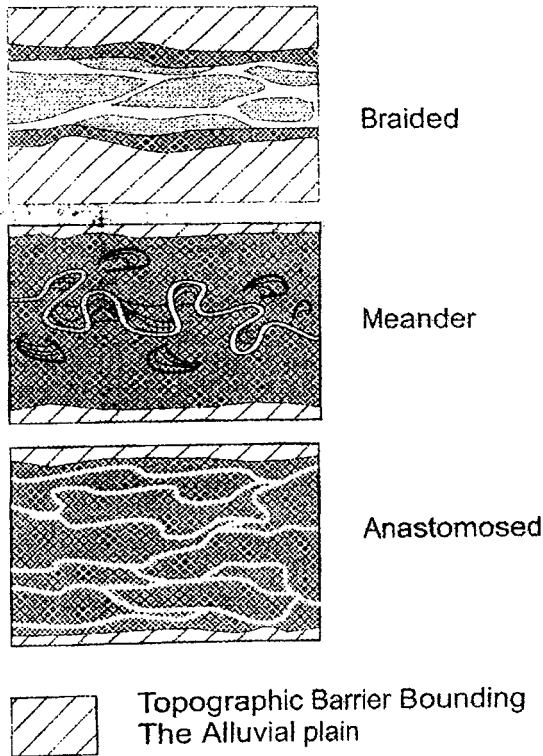
Fig. 2 Schematic representation of the principal types of natural river patterns in plan.
