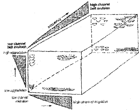
Fig. 15 Diagram illustrating the controls of different factors on the organization of channel-belt sediment bodies. Adopted from Bristow and Best (1993).
