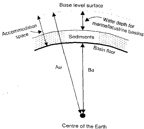
Fig. 11 Diagram illustrating definition of accommodation space in a sedimentary basin. Note that the space increases with increase in absolute base level (i.e. increase in Ab1) and subsidence (i.e. decrease in Bd).
