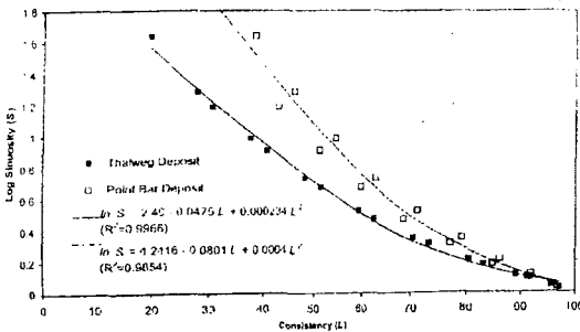
Fig. 7 Relationship between consistency and sinuosity of paleocurrent data measured from the different parts channel thalweg and bars. After Ghosh (2000).
