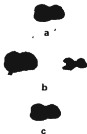
Figure 3. Enhanced/thresholded versions of chromosome for dh = 4 . (a) Algorithm 1 ( I_c = 40 ); (b) Algorithm 2 ( I_c = 29, 54 ); (c) Equation (22) ( I_c = 40 ).
