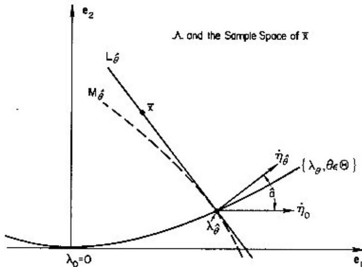
FIG. 4. A curved exponential family of dimension r - 2 . L_\theta is the set of \bar{x} for which \theta is a solution to the maximum likelihood equations. M_\theta is the level curve for another consistent efficient estimator.
