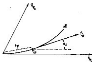
FIG. 1. The curvature of \mathcal{L} at \theta_0 is ds_\theta/ds_\theta|_{\theta=\theta_0} .
