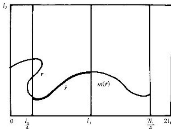
FIG. 2. The L-R crossing r of [0, l_1] \times [0, l_2] . The segment \tilde{r} of r after the last intersection with the line \{l_1/4\} \times [0, l_2] is depicted by the thick line. The reflection of \tilde{r} on \{l_1\} \times [0, l_2] is m(\tilde{r}) . The region J(r) is the region above \tilde{r} \cup m(\tilde{r}) in the rectangle [l_1/4, 7l_1/4] \times [0, l_2] .
