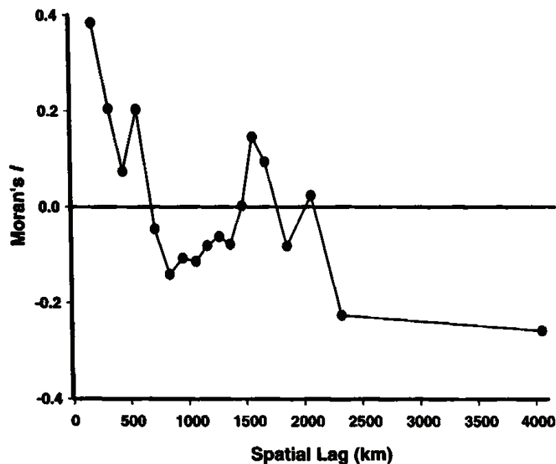
Figure 11. Spatial autocorrelation analysis. Correlogram for NI.
