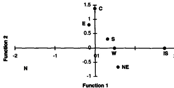
Figure 5. Discriminant functions evaluated through group centroids (geography). N, north; NE, north-east; E, east; C, central; S, south; W, west; and IS, island.
