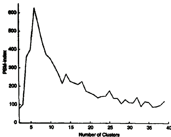
Fig. 6. Variation of the PBM-index with the number of clusters for Circular. 6.2.
