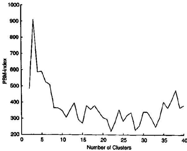
Fig. 12. Variation of the PBM-index with the number of clusters for Kalazaar .
