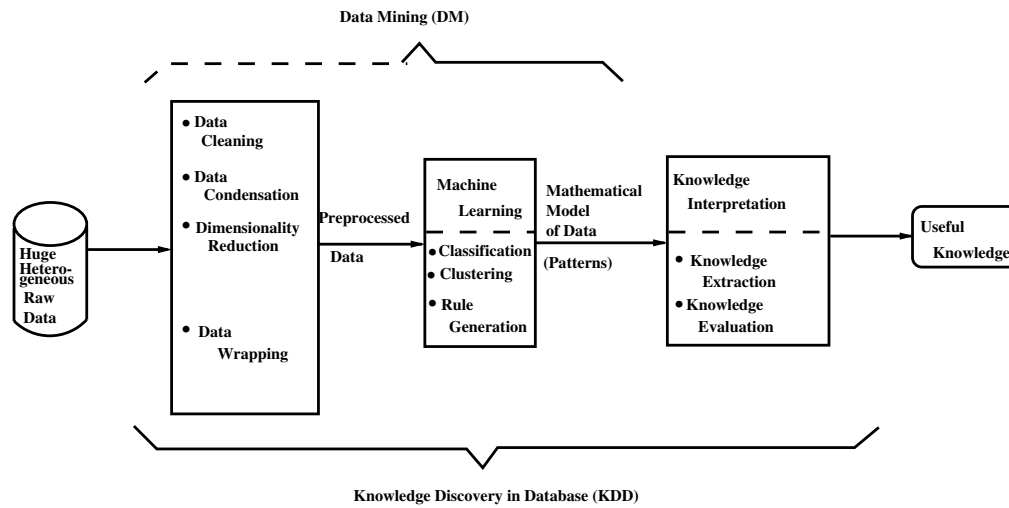
Fig. 1. Block diagram for knowledge discovery in databases [3].
