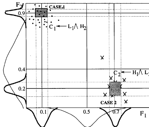
Fig. 2. Rough-fuzzy case generation for a two-dimensional data [15].
