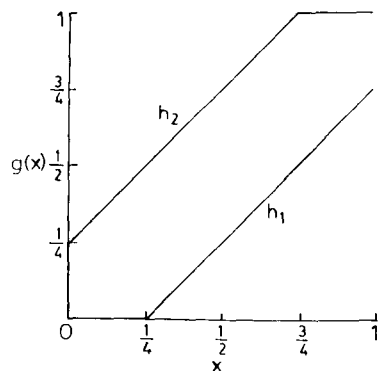
Figure 7. Bound functions.
