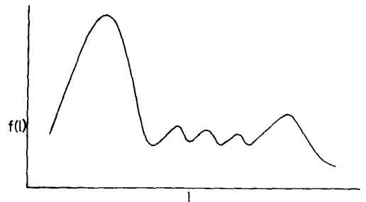
Figure 3. Histogram where convexity and symmetry properties are not satisfied.
