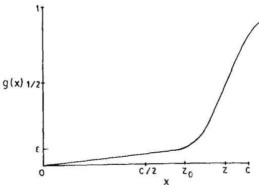
Figure 6. Membership function of Note 3.
