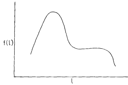
Figure 2. Histogram in which a mode can not be precisely denoted.
