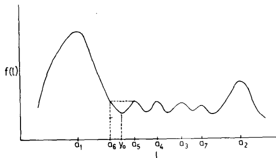
Figure 4. Histogram of Examples 1 and 2.
