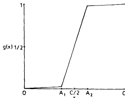
Figure 5. Membership function of Example 2.
