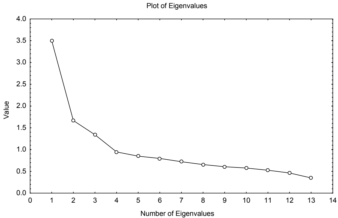
Figure: 5.2 Scree Plot of Principal Components
